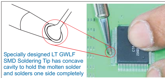
WP 80 Soldering Iron
